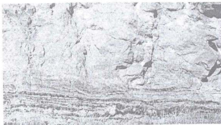
Fig. 7: Base of rhyolite lava flow with obsidian bands at sample site JI-09 on Jebel Isbil
