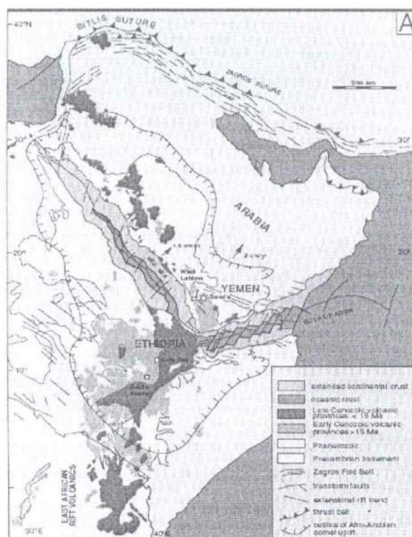
Fig. 2: Cenozoic volcanism in the Afro-Arabian province. From Ukstins-Peate et al., 2005
